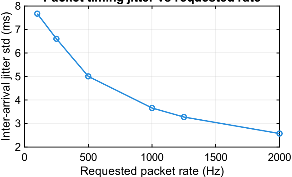
Packet timing jitter vs requested rate
